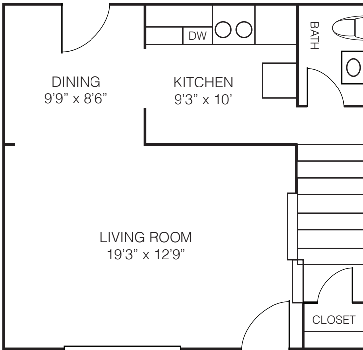
1ST FLOOR LEVEL
