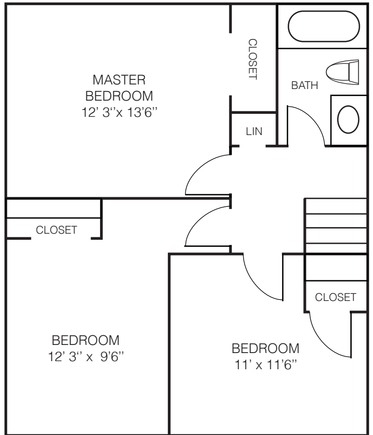
2ND FLOOR LEVEL
